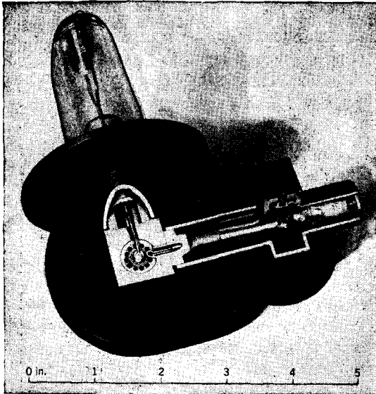
FIG. 5-2.—Halo-loop coupling.
